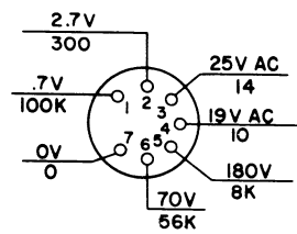
2D MIXER V205 6BE6
