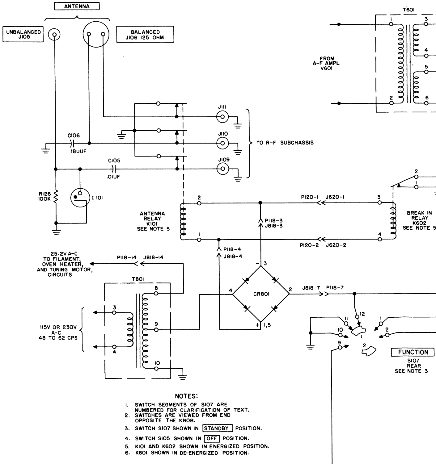
Figure 41. Break-in circuit
