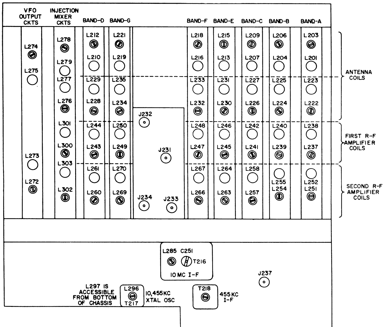
Figure 77. Location of rf alinement adjustments.
