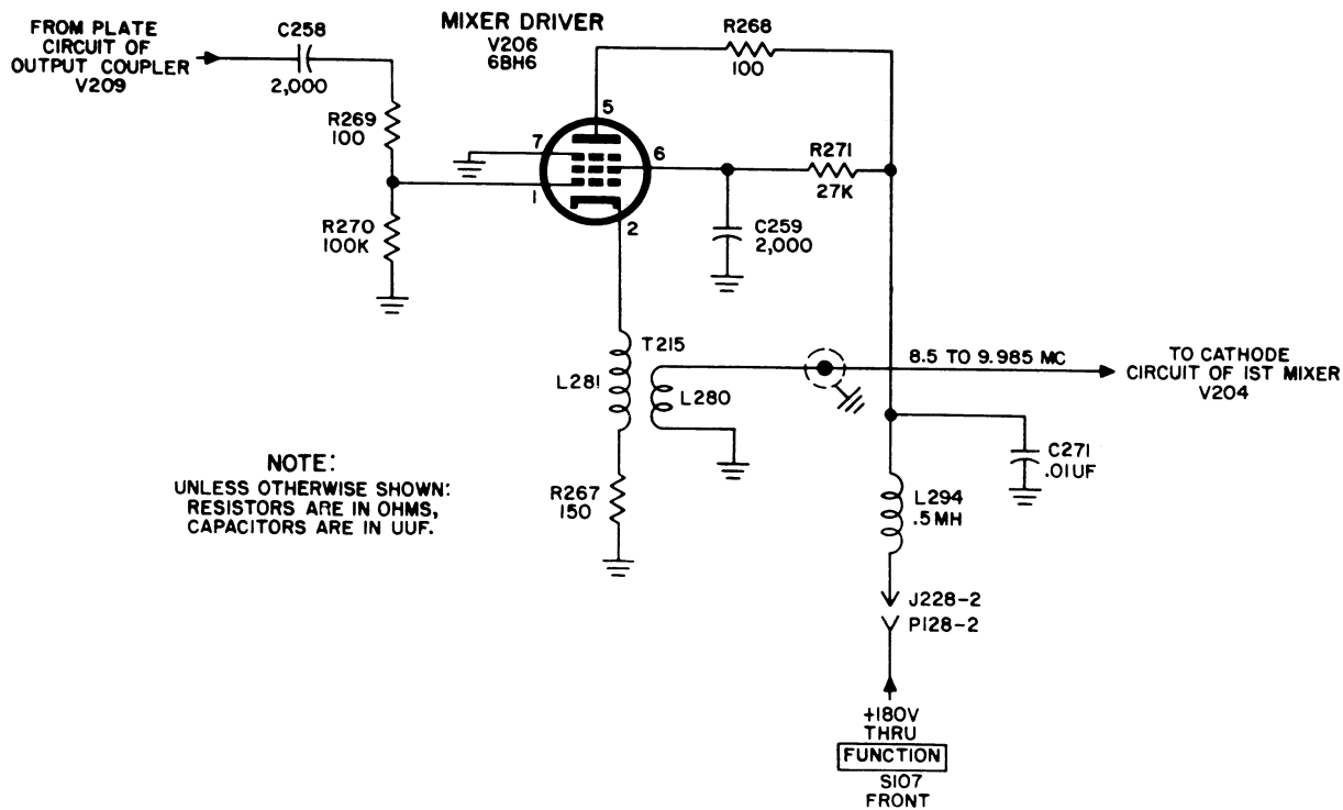
Figure 22. Mixer driver, schematic diagram.
